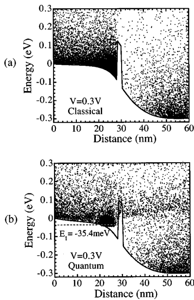
FIG. 4. Self-consistent solutions of electron distribution in space and energy at bias voltage of 0.3 V. The barrier width is 2.5 nm. (a) corresponds to the classical MC simulation and (b) to the quantum-corrected MC simulation. The conduction band profiles are plotted with solid lines, and the vertical axis denotes the total electron energy, including the contribution of quantum force (quantum potential).
