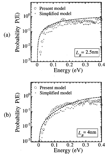
FIG. 3. Computed tunneling probabilities as a function of energy for simulation conditions as in Fig. 1 with barrier width (a) 2.5 and (b) 4.0 nm. The shaded areas indicate the energy range above the barrier ( E > 0.22 eV). The open circles denote the result from the correction model of Eq. (27) and the crosses the result from the simplified correction model of Eq. (23). For comparison, the results from a transfer matrix solution of Schrödinger equation are plotted with the dashed lines.
